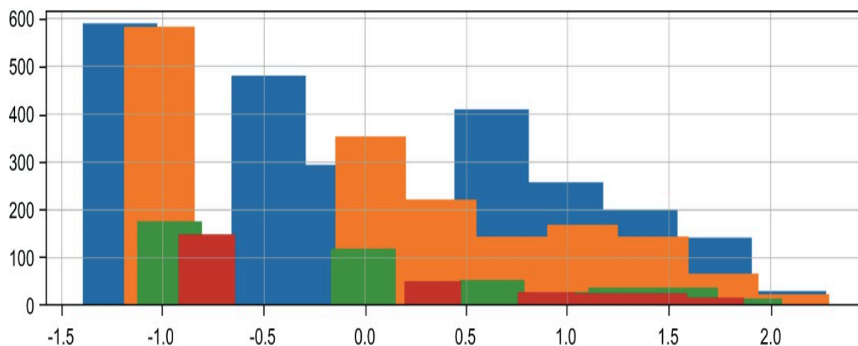
Figure 4.18 After applying the Yeo-Johnson transformation on each subgroup’s subset of priors counts, the distributions begin to look much less skewed and different from one another. This will make it difficult for the ML model to reconstruct race from this feature.
