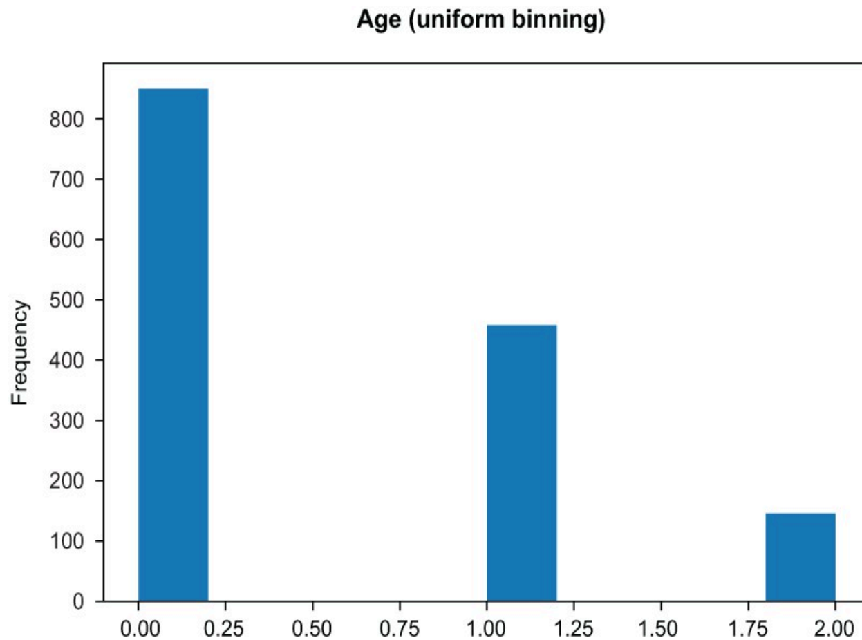
Figure 3.13 Uniform binning yields bins of equal width.
