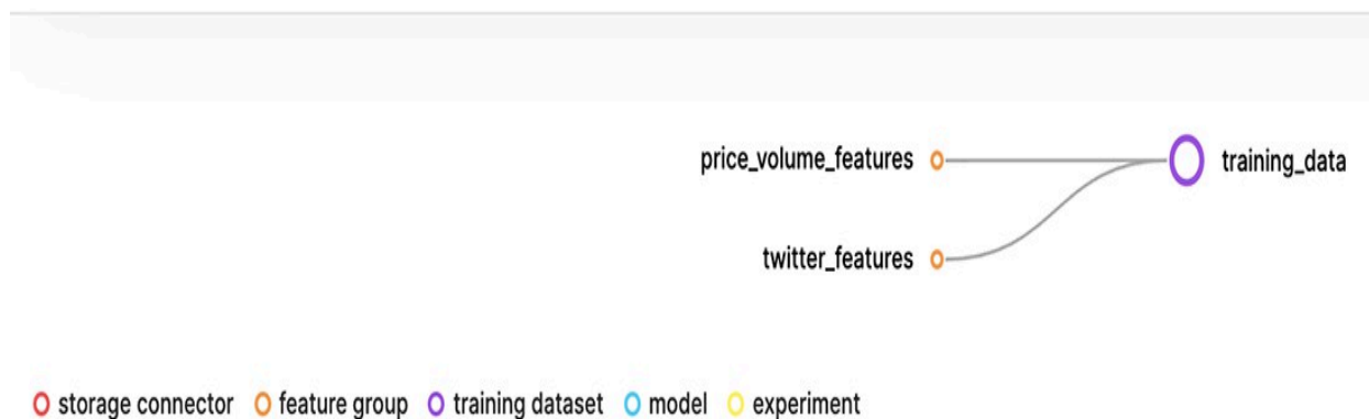
Figure 8.20 An example of a provenance (lineage) graph for our training dataset and the source feature groups in Hopsworks
