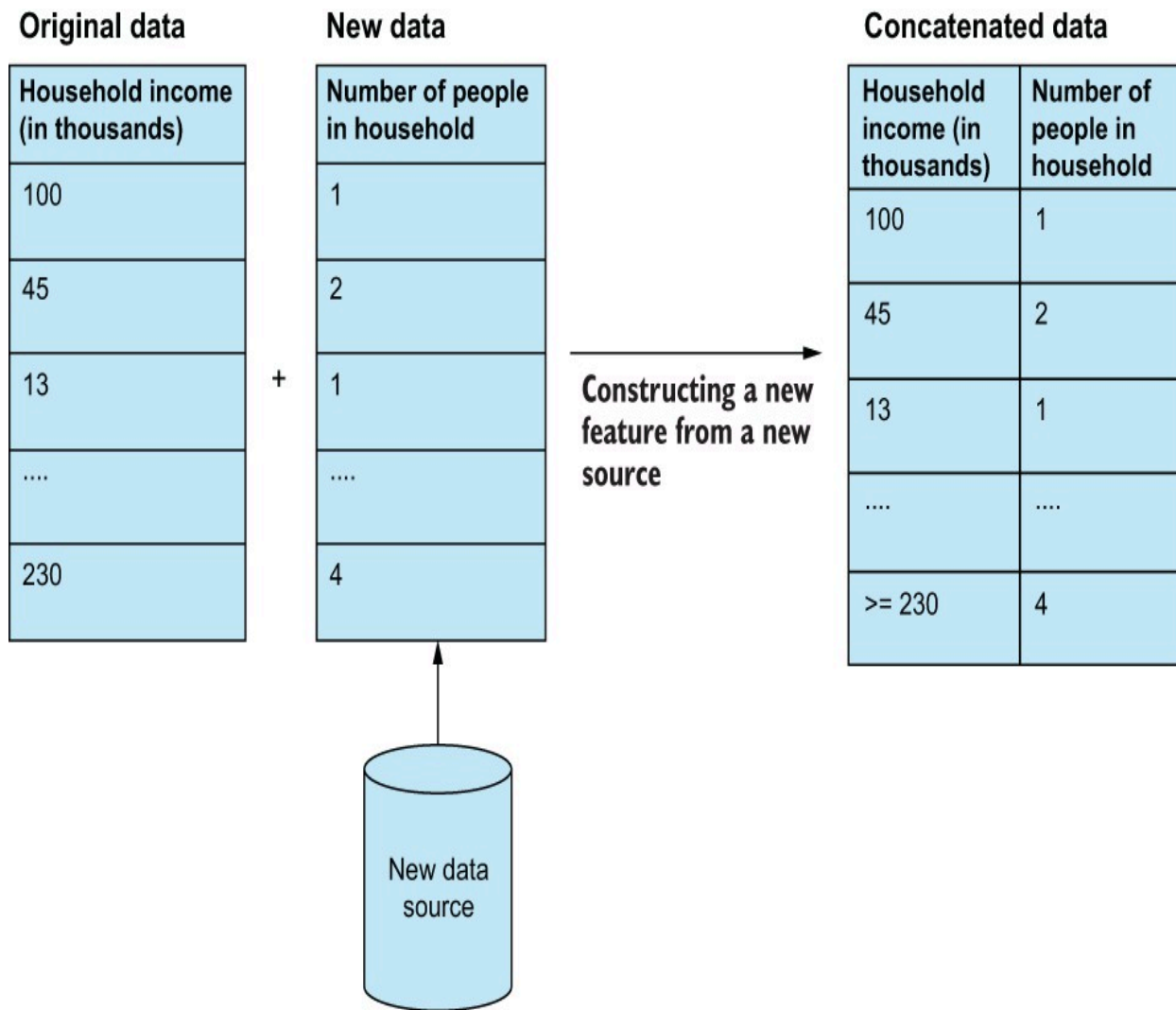
Figure 2.8 Feature construction often refers to concatenating new features from a new data source that is different from the source of the original dataset. The difficulty in this process often lies in merging the old and new data to make sure they align and make sense.
