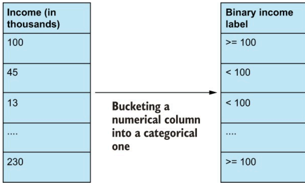
Figure 2.9 Feature construction also can look like feature improvement, wherein we apply some transformation to an existing feature. The difference here is that after applying the transformation, the interpretability of the feature drastically changes. In this case, we've changed the original numerical income feature to be a new categorical bucketed feature. The same information is generally there, but the machine learning algorithms must now process the feature in an entirely new way on an entirely new dimension.
