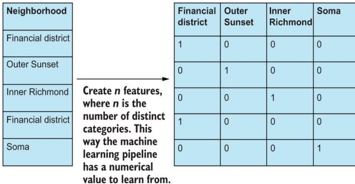
Figure 2.2 Creating dummy binary features from nominal features. We could also have chosen n \times 1 features to dummify, as it is implied that if the rest of the values are 0, then the n th feature would be a 1.
