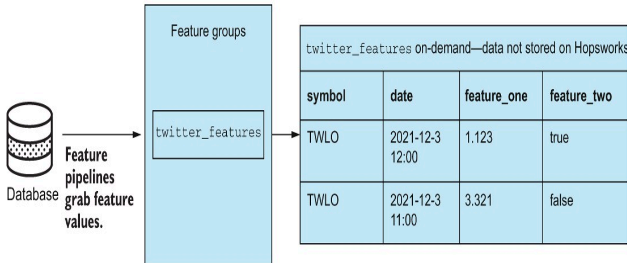
Figure 8.10 An on-demand feature group twitter_features will grab data from the connecting database (e.g., MySQL or S3) whenever the user requests the data and will not store any values on Hopsworks.
