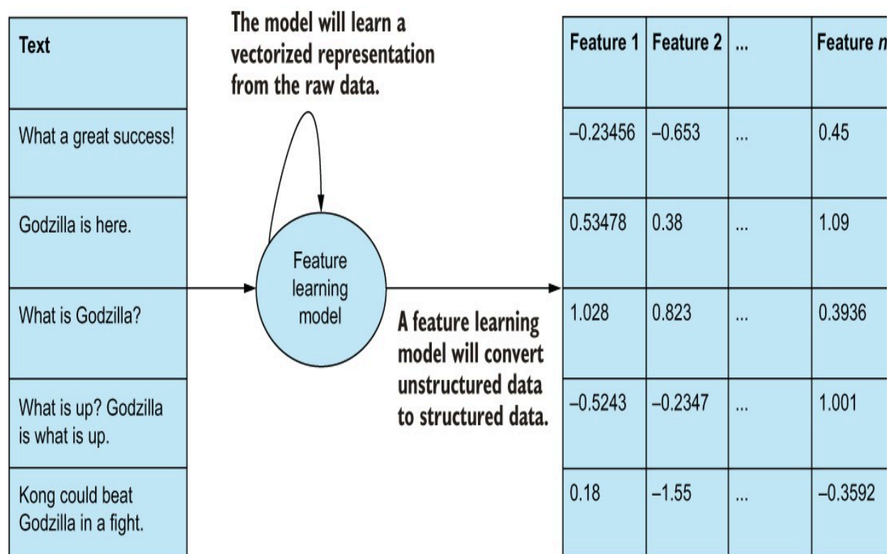
Figure 2.12 Often considered the most difficult feature engineering technique, feature learning is the process of learning an entirely new set of features, usually by way of some nonparametric feature learning model, like an autoencoder (which we will use in our NLP case study) or generative adversarial networks (which we will see in our Image case study).
