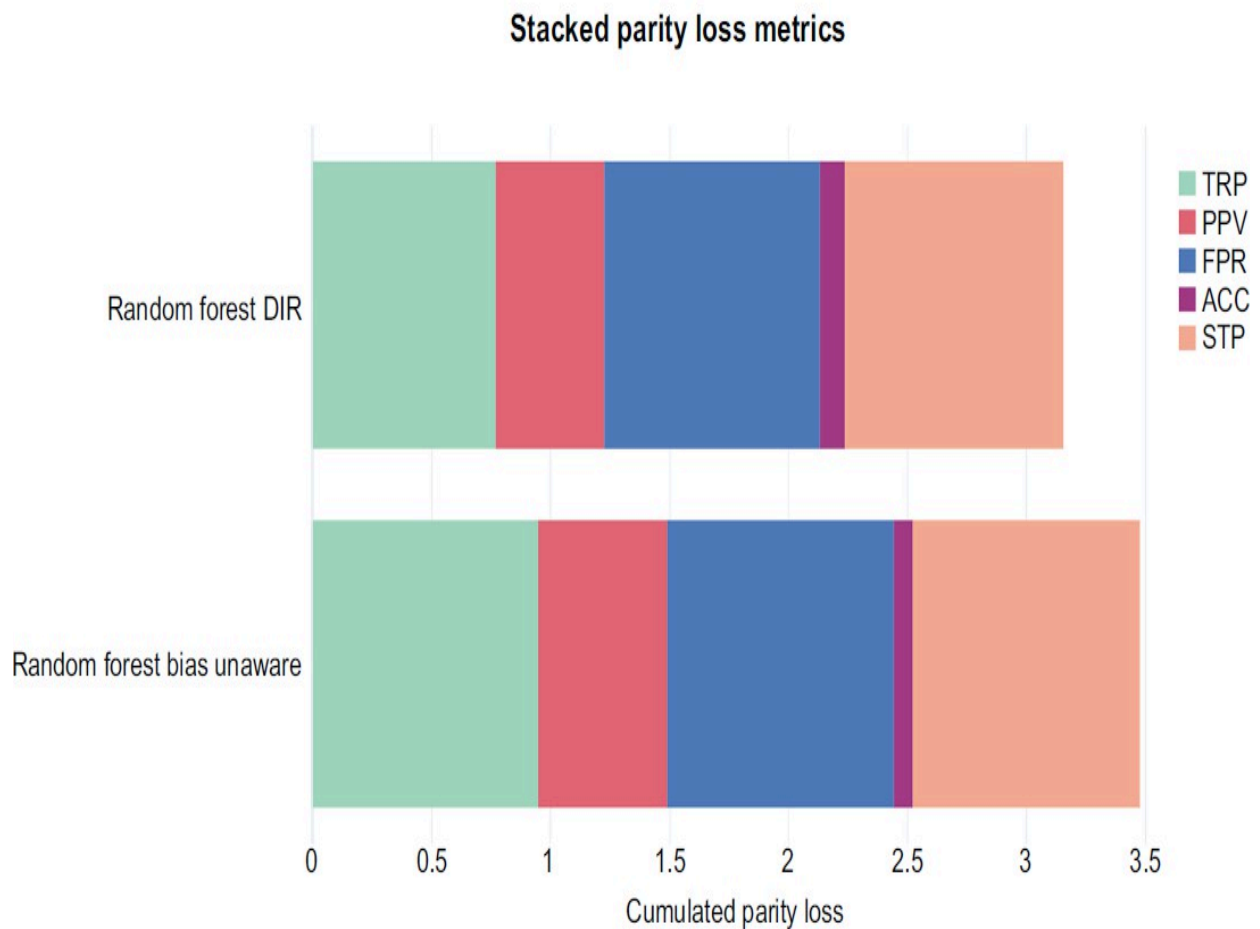
Figure 4.19 The top bar represents the sum of our bias metrics for our bias-aware model, which is seeing a minor boost in model performance (noted in the metric table) in all metrics, except recall, where it is unchanged. The bottom bar shows the original bias-unaware stacked plot we saw earlier. Overall, our new bias-unaware model is performing better in some ML metrics and is showing a decrease in bias based on our parity loss bar chart. We are on the right track!
