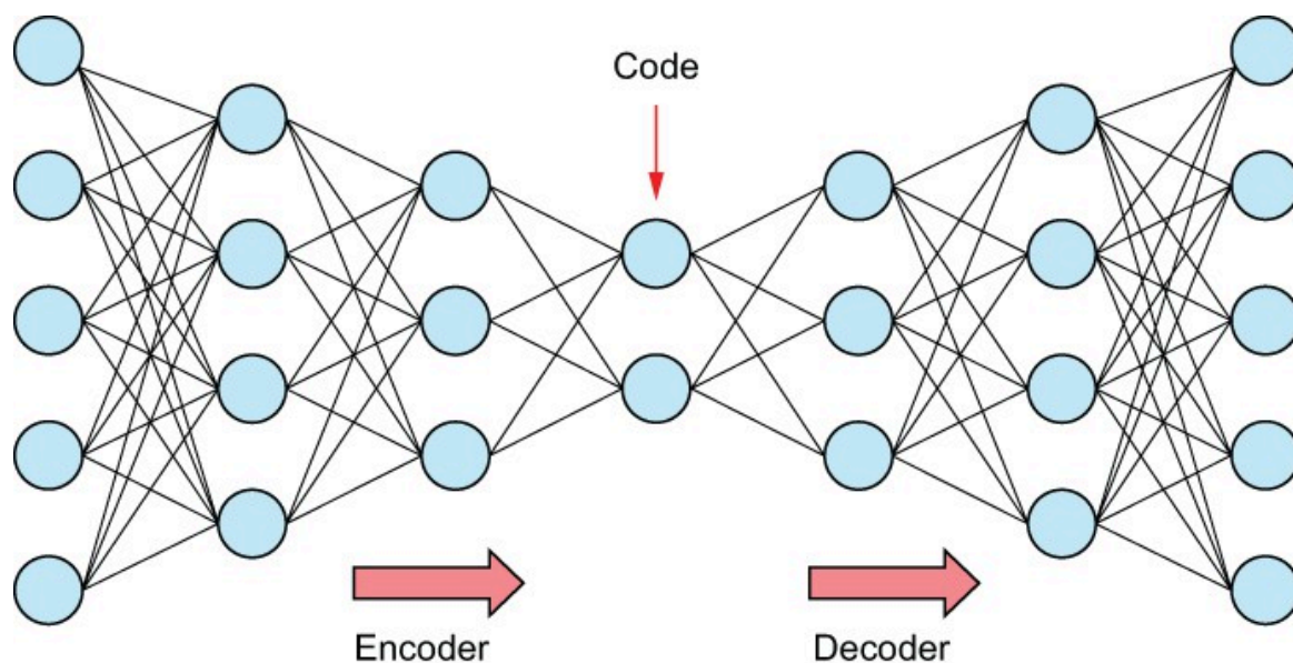
Figure 5.23 Autoencoders are neural networks that deconstruct and reconstruct data through a series of layers, with the middle layer called the "code" or the "bottleneck." The code/bottleneck layer is often used as a reduced-size latent compression of the input data.
