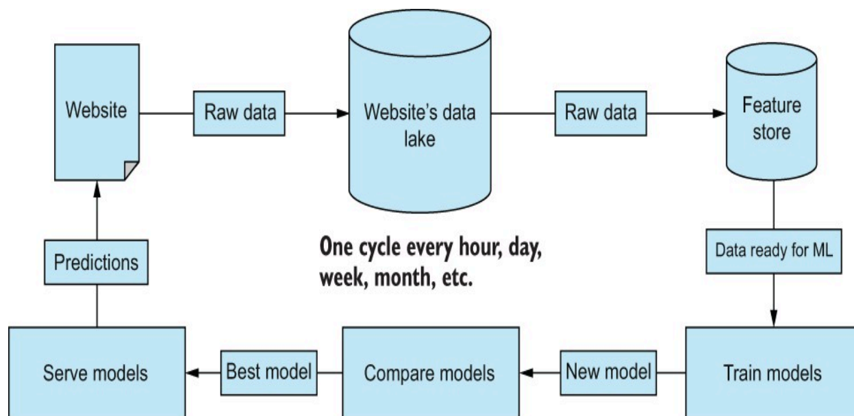
Figure 8.4 The Wikipedia roadmap explains how they are aiming for stronger MLOps to attract more users with accurate predictions, which, in turn, will generate new data to update its models with.
