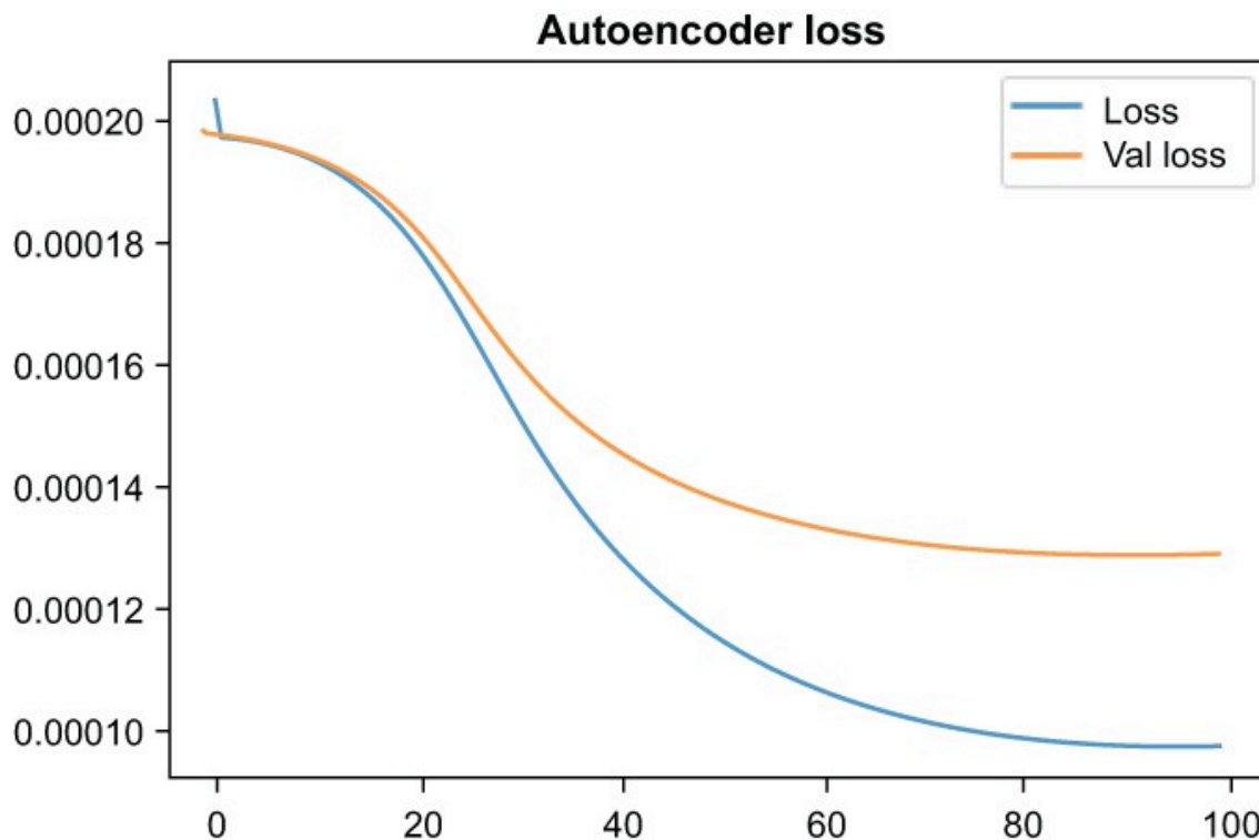
Figure 5.25 Our autoencoder is able to deconstruct and reconstruct TF-IDF features based on the dropping loss! Our hope is that, by doing so, the autoencoder has learned a latent set of features that will prove valuable to our ML pipeline.
