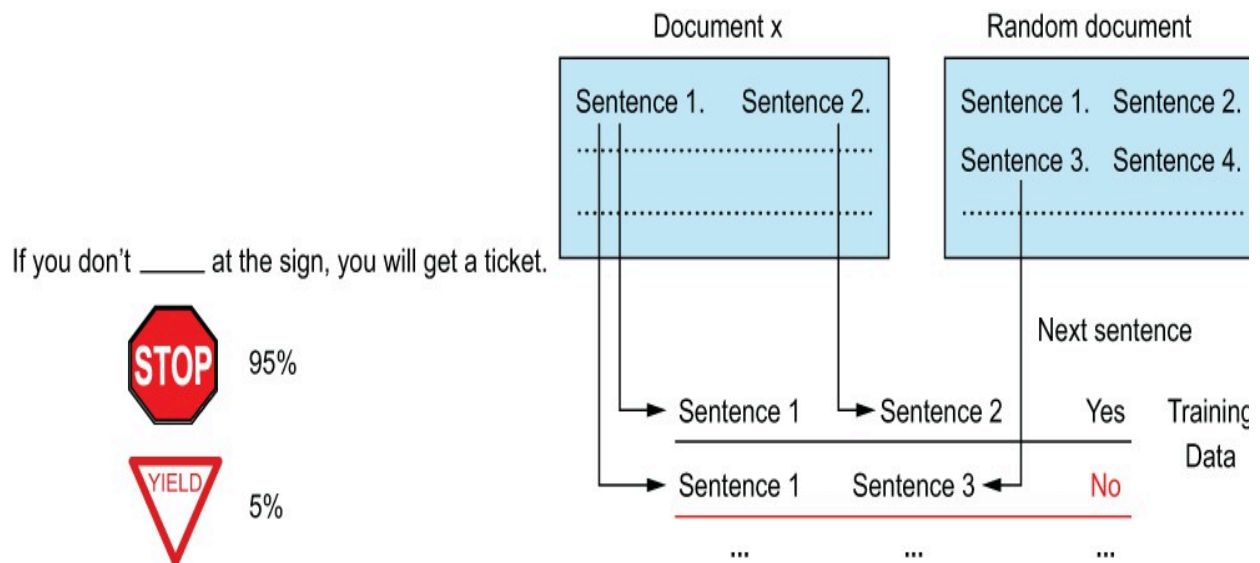
Figure 5.30 The masked language model pretraining task (on the left) teaches BERT what individual tokens mean in the context of a larger sentence. The next sentence prediction task teaches BERT how to align sentences in a larger document.
