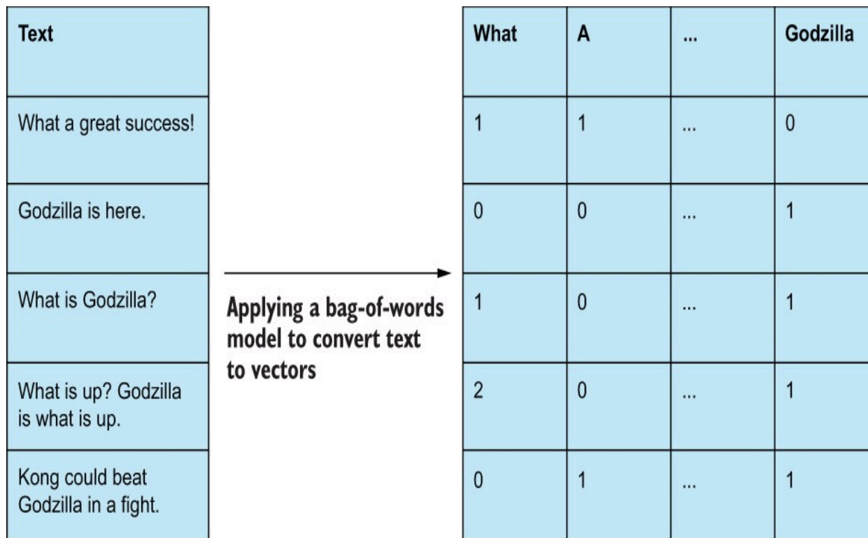
Figure 2.11 Bag-of-words models convert raw text to multi-hot encodings of word counts.
