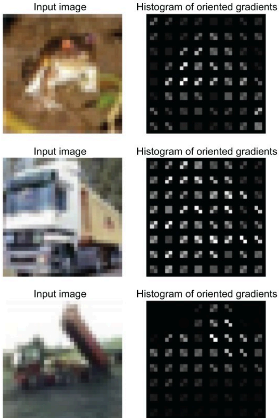
Figure 6.4 A sample of CIFAR-10 images with their accompanying HOG visualizations. Each cell shows us the most dramatic directions of movement to highlight edges in the image. The HOG visualizations are a lower-fidelity representation of their original raw images that will provide the input to our ML model.
