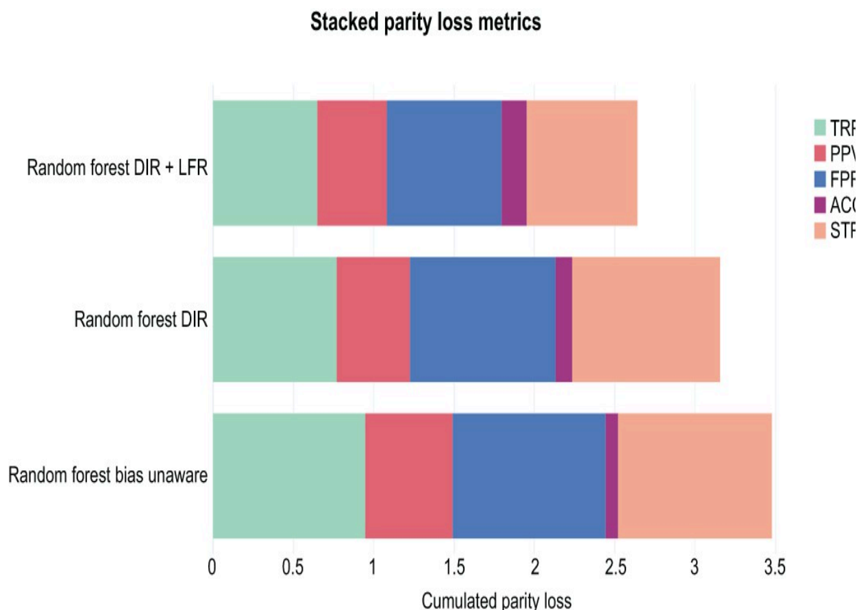
Figure 4.21 Our final, bias-aware model that has disparate impact removal and LFR is the fairest model yet. Again, keep in mind that
