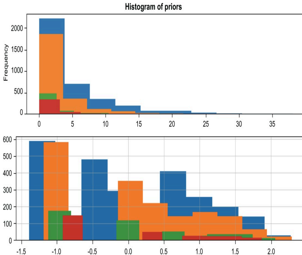
Figure 9.5 In chapter 4, we applied the Yeo-Johnson transformation to our original data (above) to create a new distribution of prior counts (below), making it difficult for our ML pipelines to draw correlations between protected features, like race, and features like priors counts. In our dataset, folks who identified as African American had more priors counts than the rest of the people in the dataset. That opened the door for bias to be introduced by reconstructing race from previous counts.
