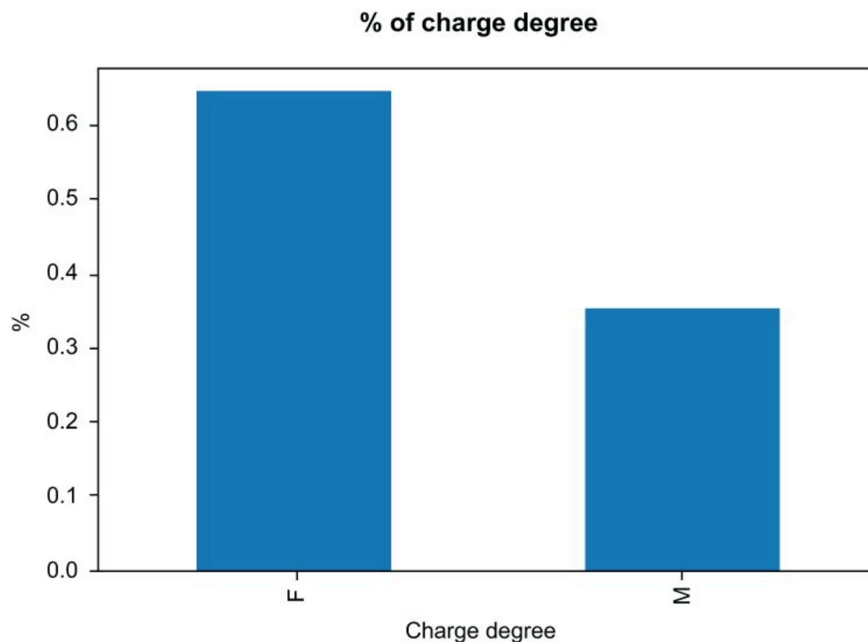
Figure 4.6 Distribution of felonies and misdemeanors in our dataset by degree. We have about 65% of our charges as F for felonies, and the
