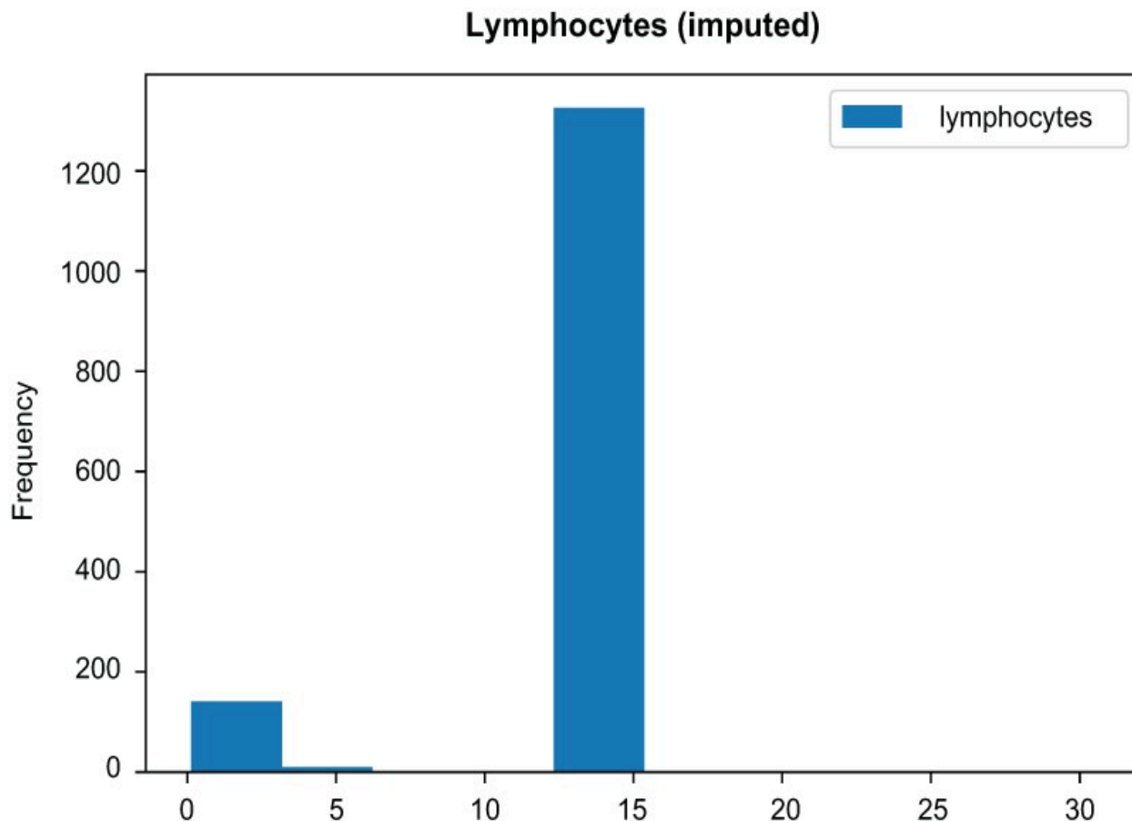
Figure 3.5 The lymphocytes feature after applying end-of-tail imputation
