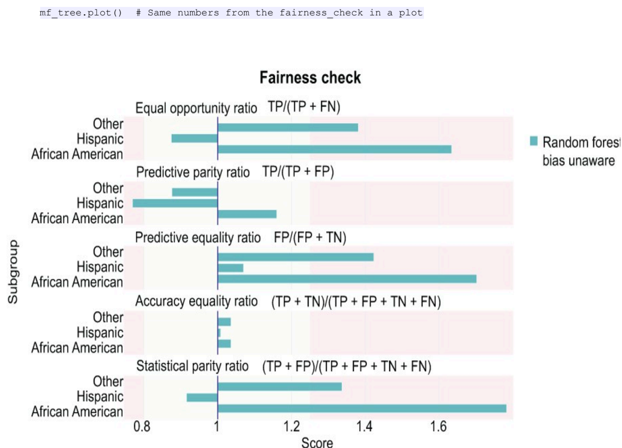
Figure 4.14 Dalex offers a visual breakdown of the five main ratios we will focus on, broken down by subgroup. The lighter areas of the bars are meant to convey acceptable ranges for fairness. Any bar in the darker regions are out of range of (.8, 1.25) and are considered unfair. We can see that we have some work to do!
