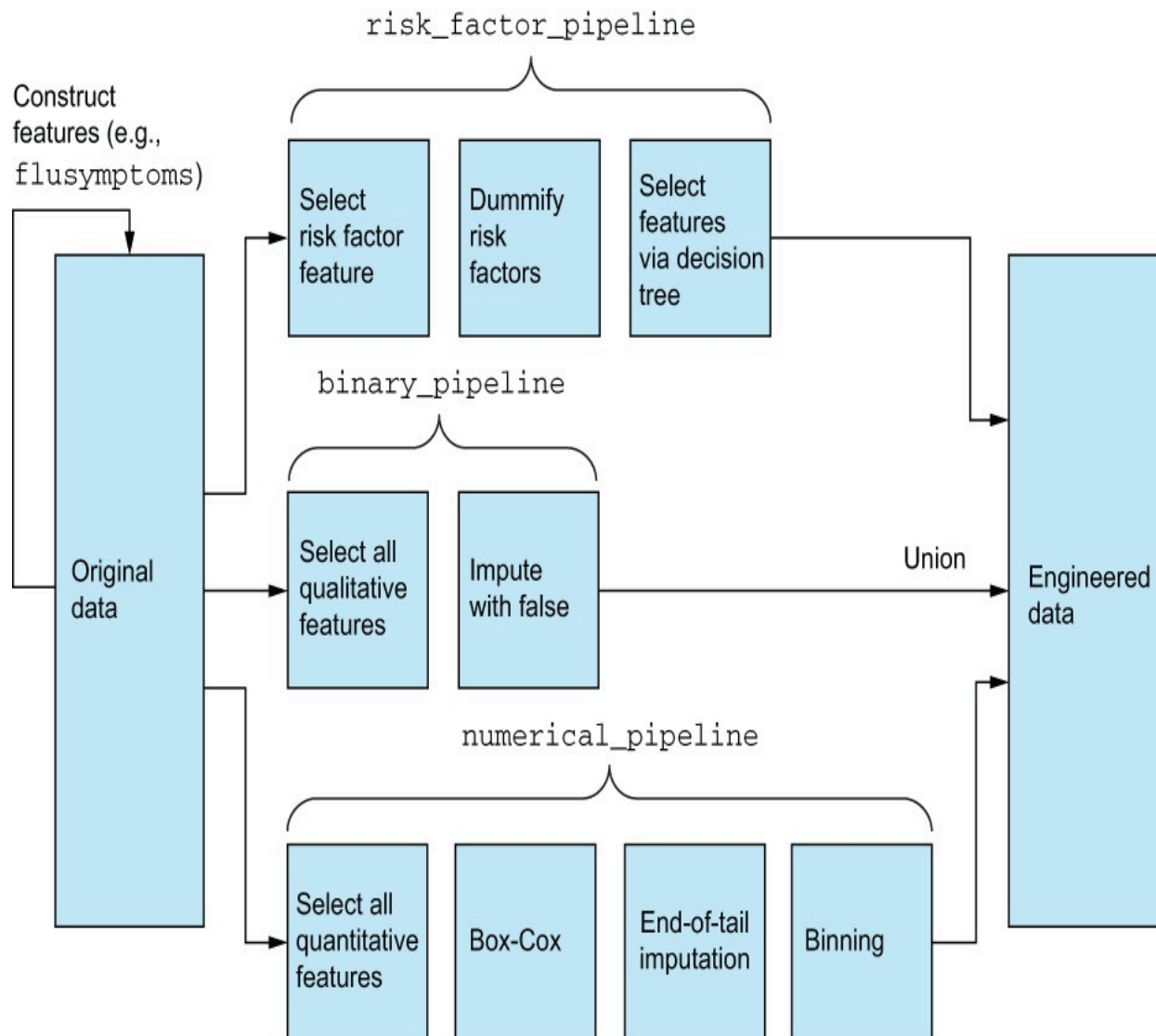
Figure 3.30 Our final feature engineering pipeline
