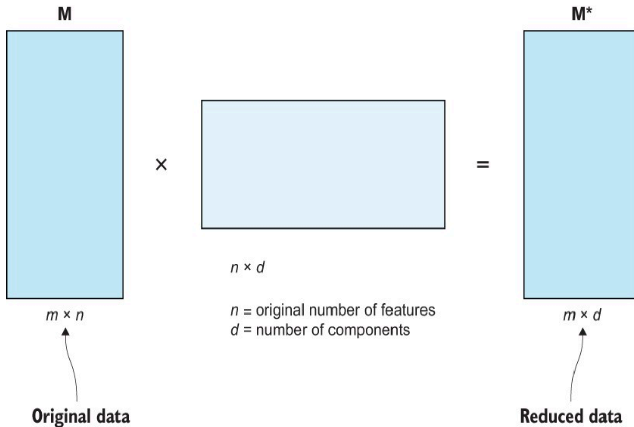
Figure 5.21 Using SVD to perform dimension reduction allows us to reduce the number of token features ( n ) into a latent smaller number of features ( d ).
