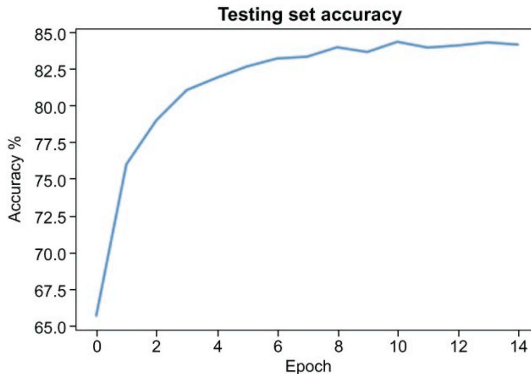
Figure 6.12 Fine-tuning VGG-11 peaked around 84% accuracy in the test set.
