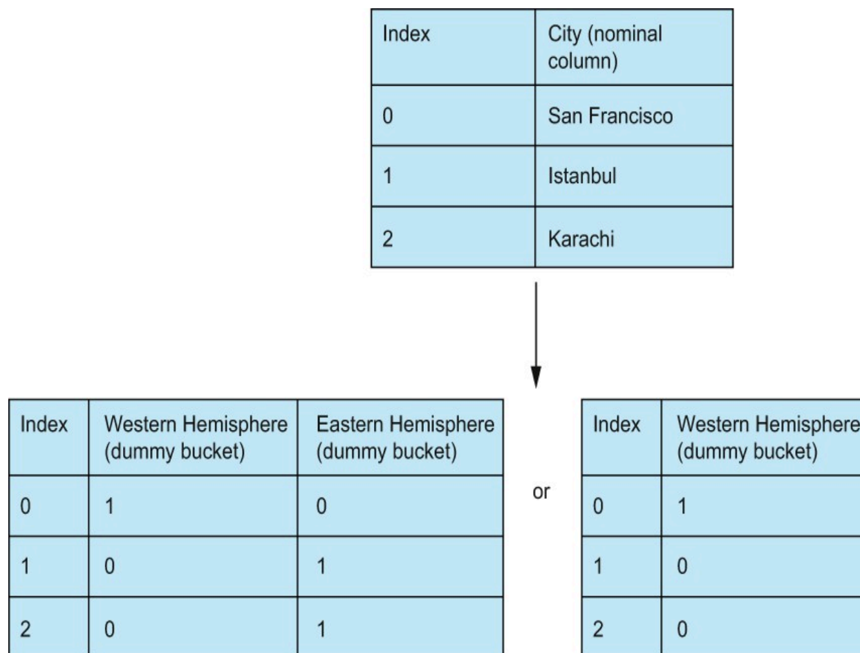
Figure 9.11 Nominal features should end up as dummy variables. In the case of two categories, I'd recommend removing one of the dummy variables because they are 100% correlated in this case. A 0 in one feature means the other feature is 1.
