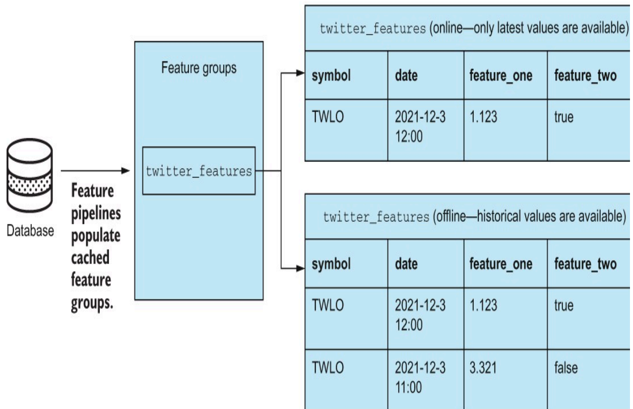
Figure 8.9 A cached feature group twitter_features that is available both online and offline. Only the most recent information about a stock entity is stored in the online version. In the offline version, we can see the historical values for all of our Twitter features.
