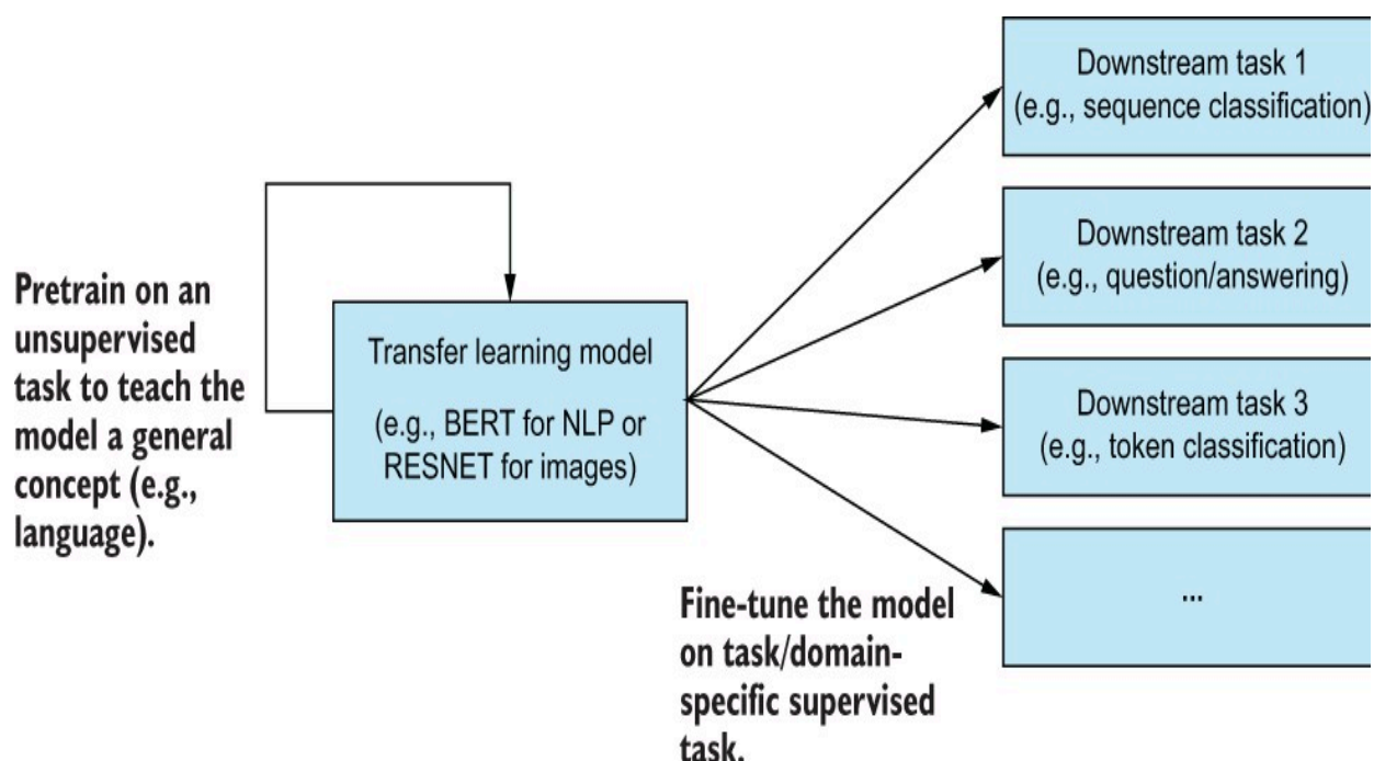
Figure 9.7 We relied on learned features from BERT in chapter 5 to obtain our best ML performance for sequence classification.
