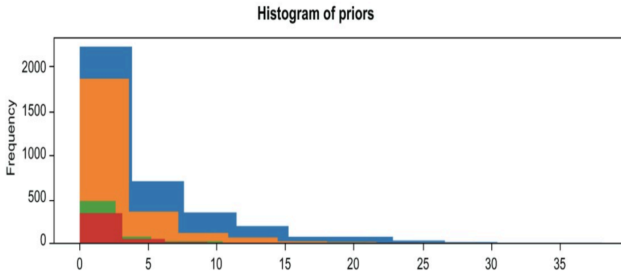
Figure 4.17 At first glance, it may seem like the patterns of priors for all races are similar. Distributions of priors count show a similar right skew between racial groups. However, for reasons out of many people’s control, the median and mean priors counts for African Americans are nearly twice that of the other groups.
