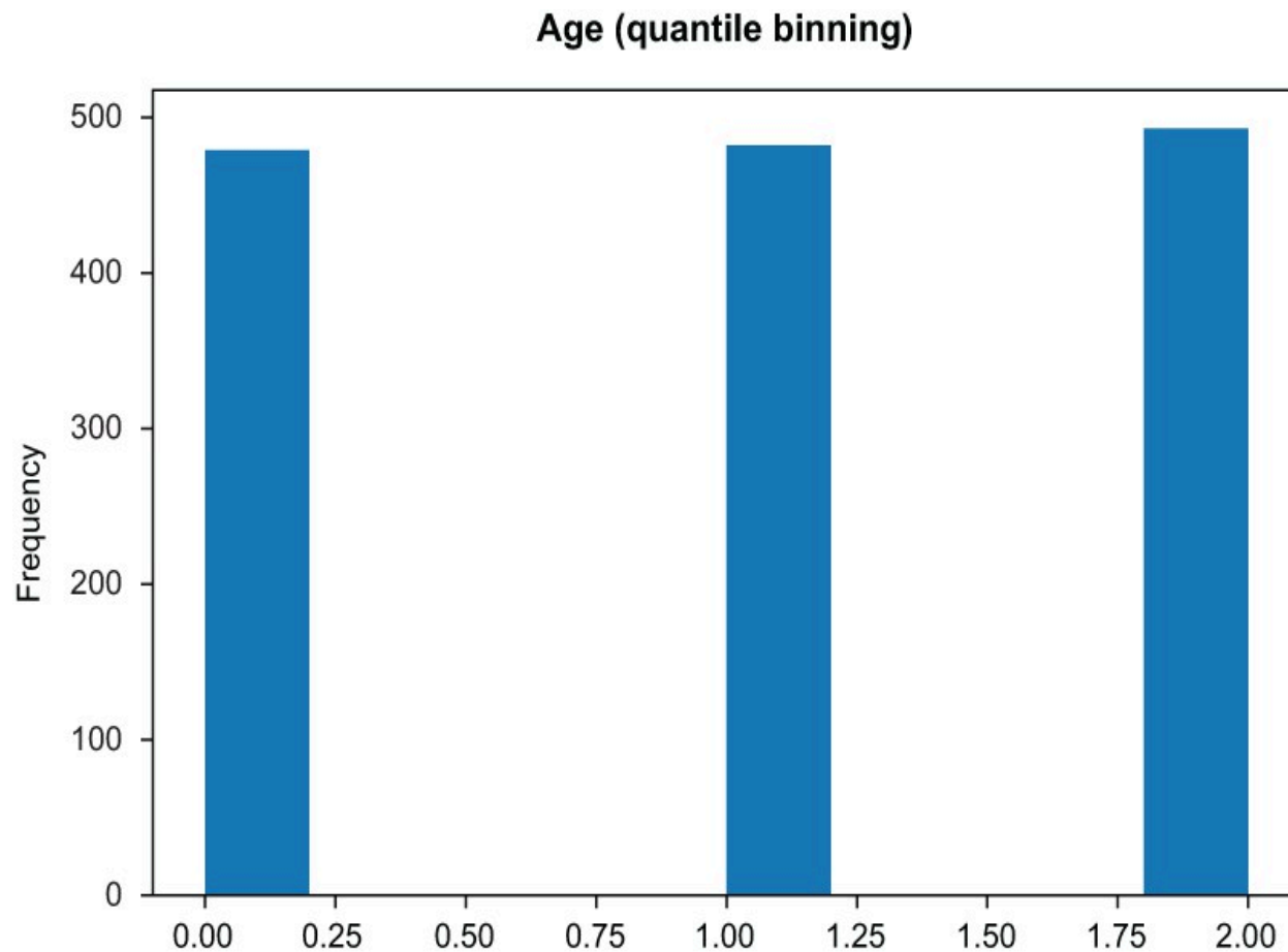
Figure 3.14 Quantile binning yields bins of equal height.
