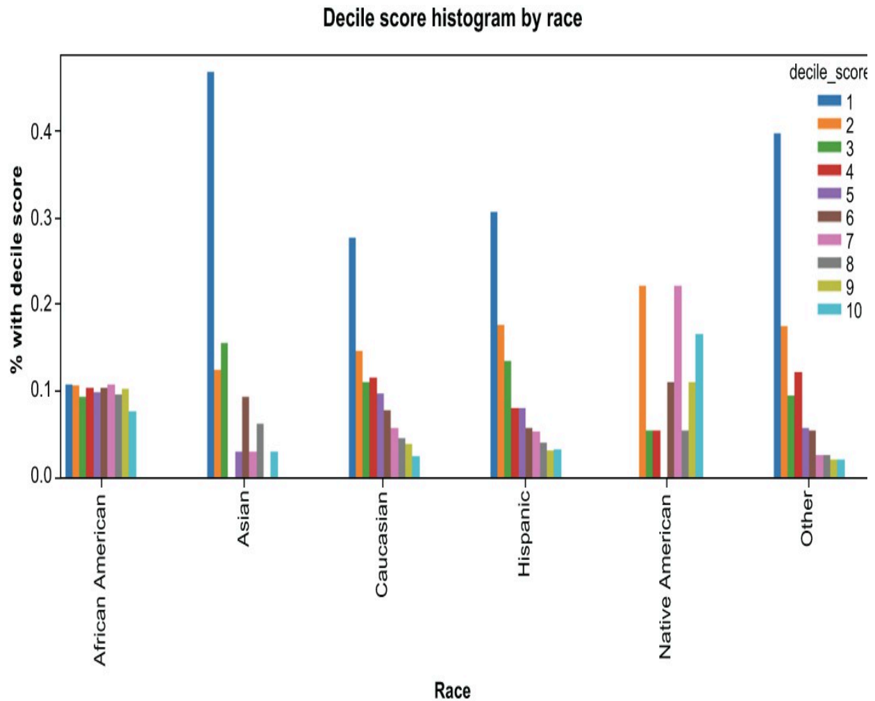
Figure 4.2 We can see clear differences in how decile scores are distributed when broken down by race.
