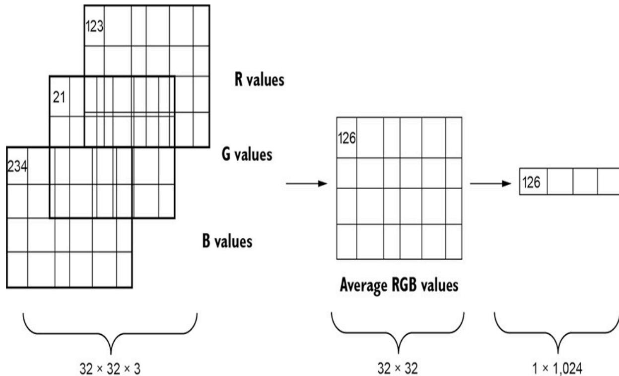
Figure 6.2 The MPV approach converts images into arrays by averaging the red, green, and blue pixel matrices into a single matrix of averaged color values and then realigning the average-color matrix to be a single dimension per image.
