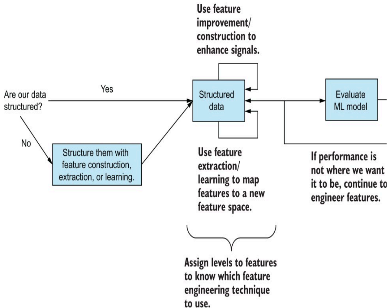
Figure 2.13 A high-level pipeline of how we will approach feature engineering in this book
