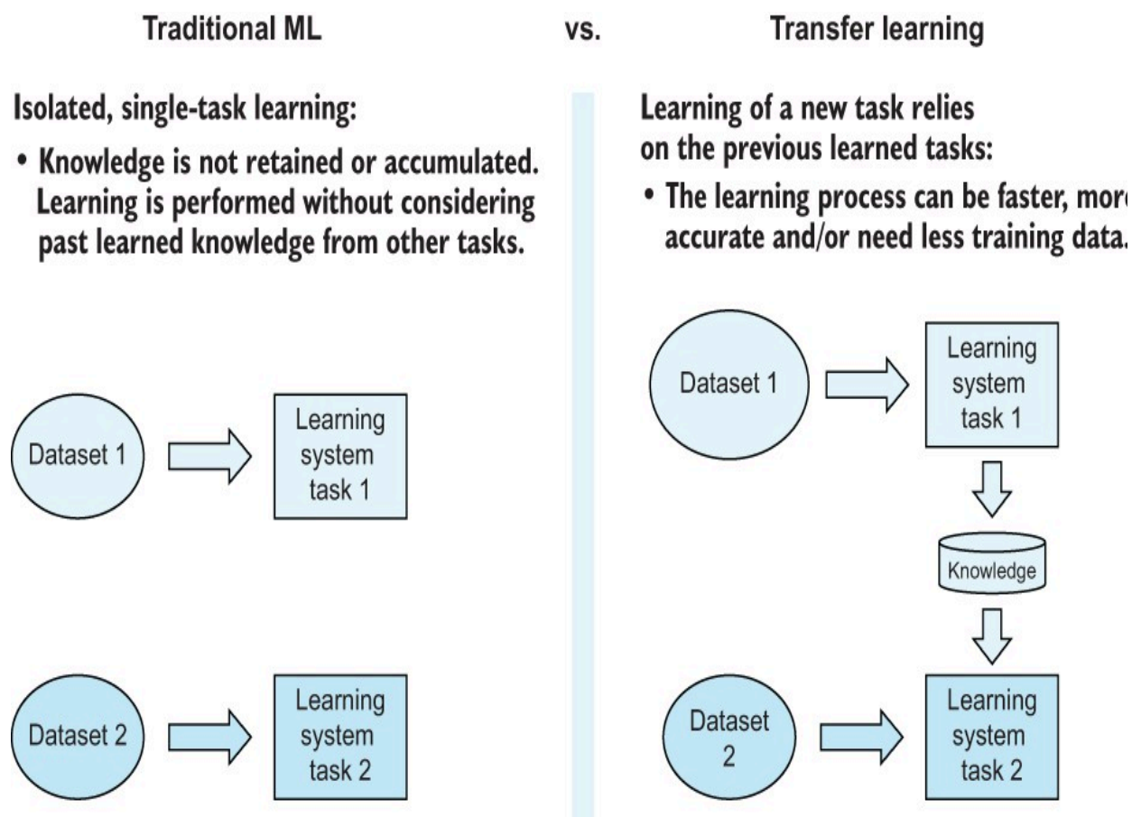
Figure 5.27 Transfer learning aims to preteach an ML model the basics of a task before giving it a second smaller dataset to fine-tune its knowledge.
