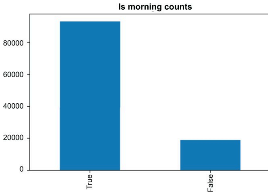
Figure 7.5 Our two date/time features give us a likely small but potentially useful signal in the way of assuming there is some
