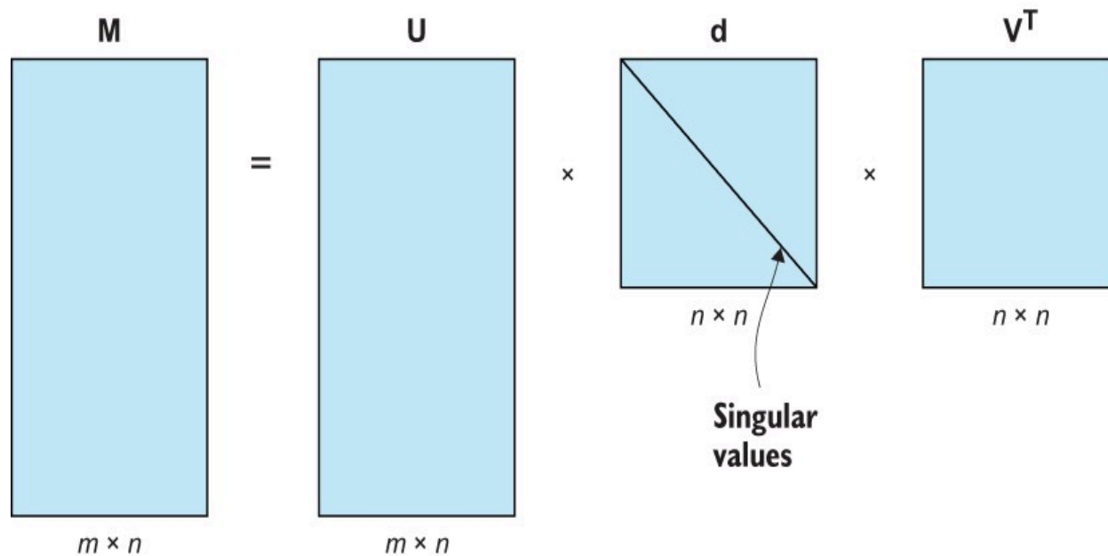
Figure 5.20 Singular value decomposition decomposes any matrix into three matrices that each represent a different linear transformation.
