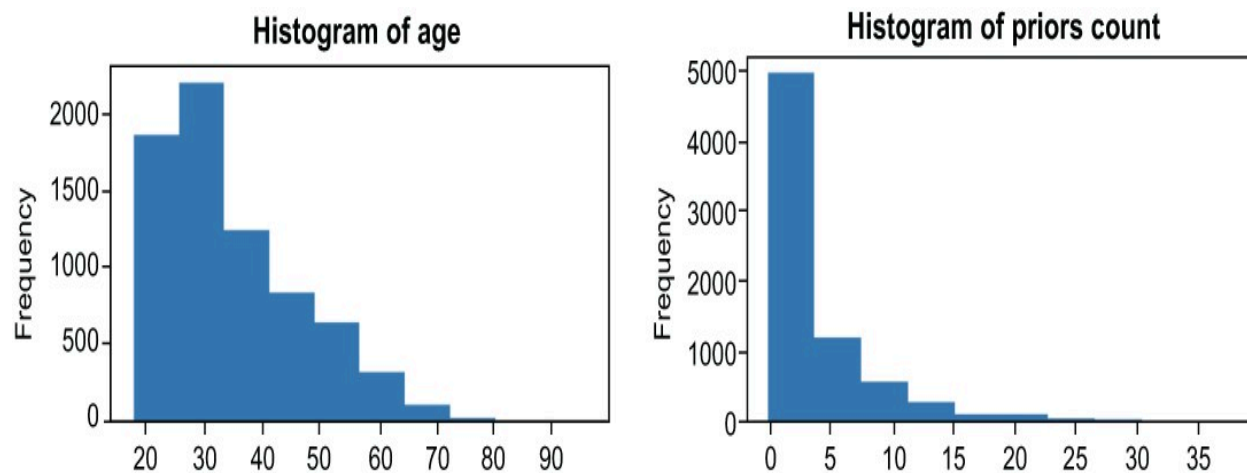
Figure 4.7 Age and Priors Count are showing a right skew in the data. It's showing that most of the people in our dataset are on the young side, but we do have some outliers pulling the average to the right. This will come up again when we investigate model fairness.
