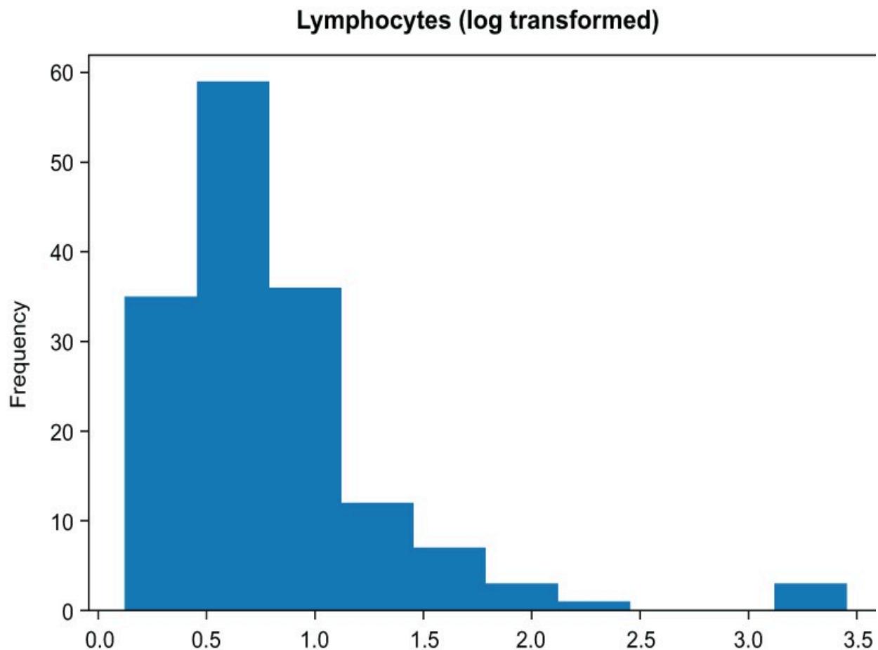
Figure 3.7 Histogram of the lymphocytes columns after applying a log transform. The data are much more normal.
