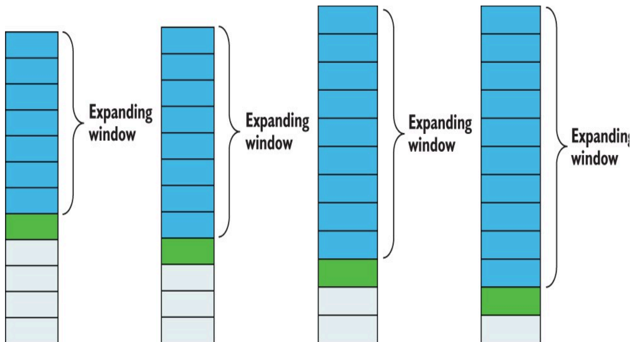
Figure 7.9 Expanding-window features use values from previous rows in an expanding window that starts from the beginning. For any given row (just below the darkest shaded rows), we use all past values (the darkest shaded rows) to calculate our expanding-window feature.
